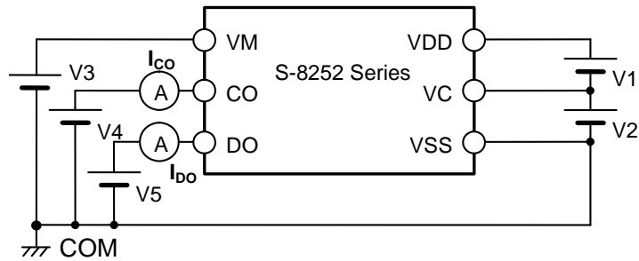
Figure 8 Test circuit 4
