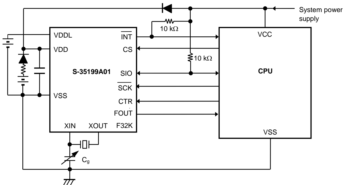
Figure 52 Application Circuit 1
