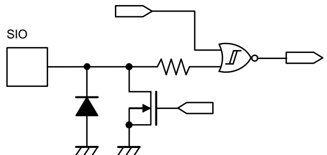
Figure 4 SIO pin
