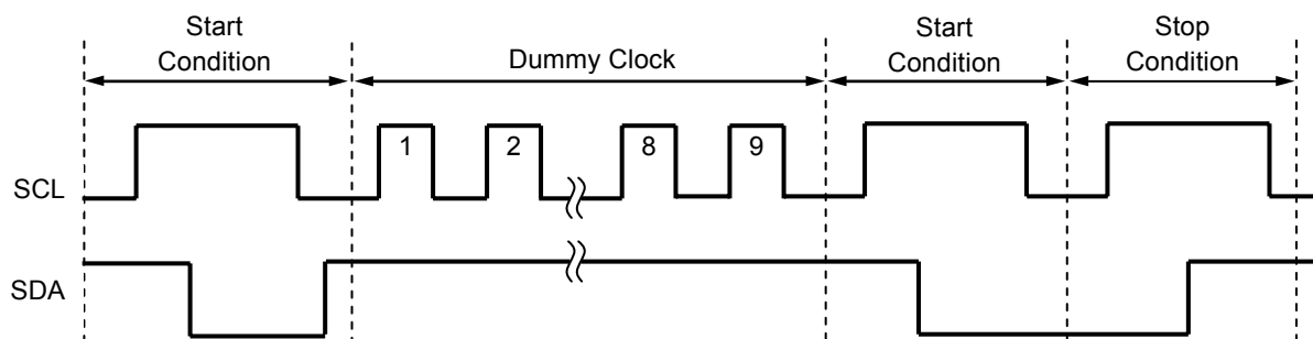
Figure 24 Resetting S-24C128C
