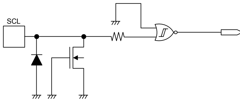
Figure 20 SCL Pin
