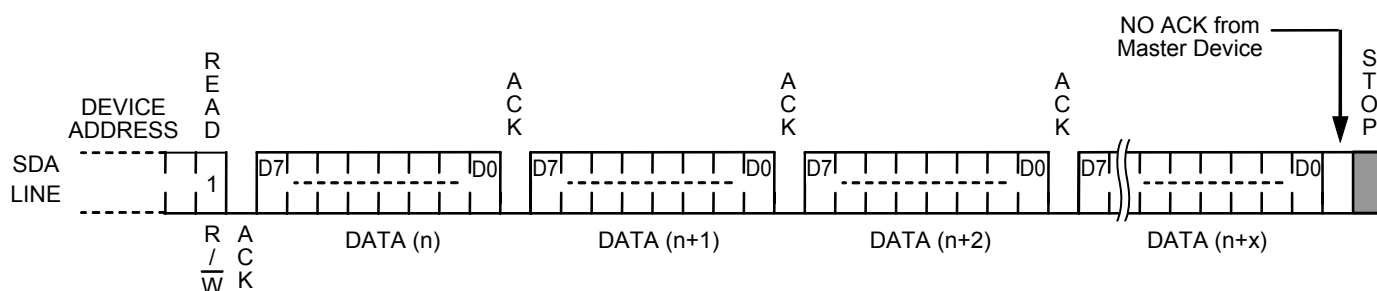
Figure 18 Sequential Read
