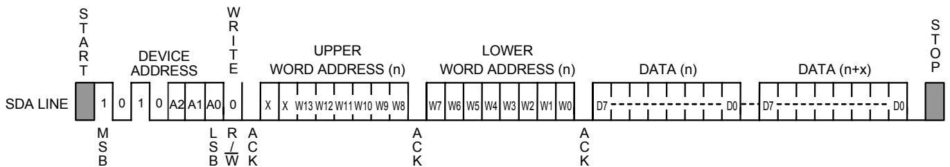
Figure 13 Page Write
