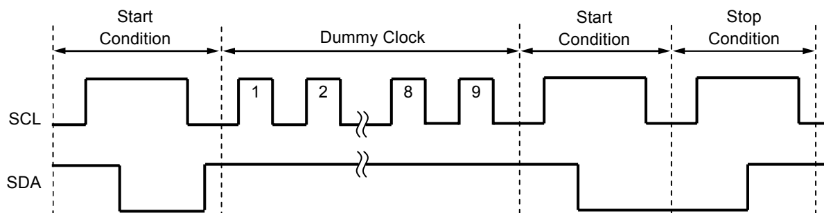
Figure 24 Resetting S-24C32C/64C
