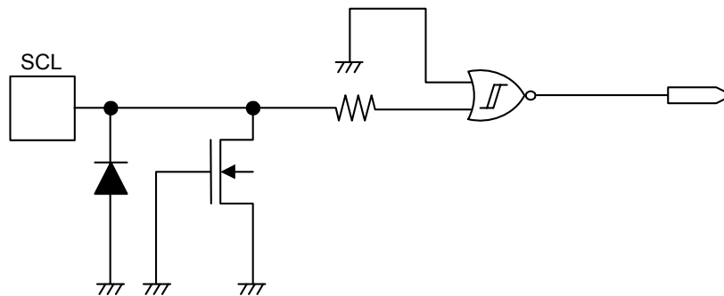
Figure 20 SCL Pin
