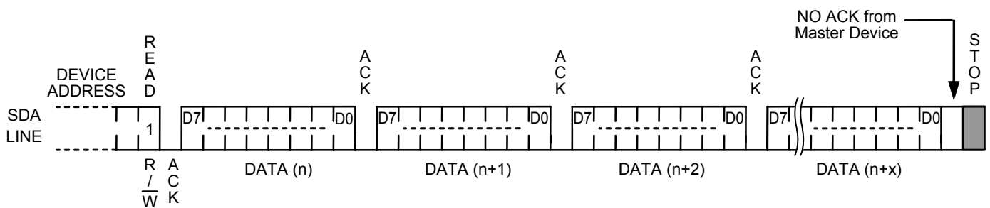
Figure 18 Sequential Read
