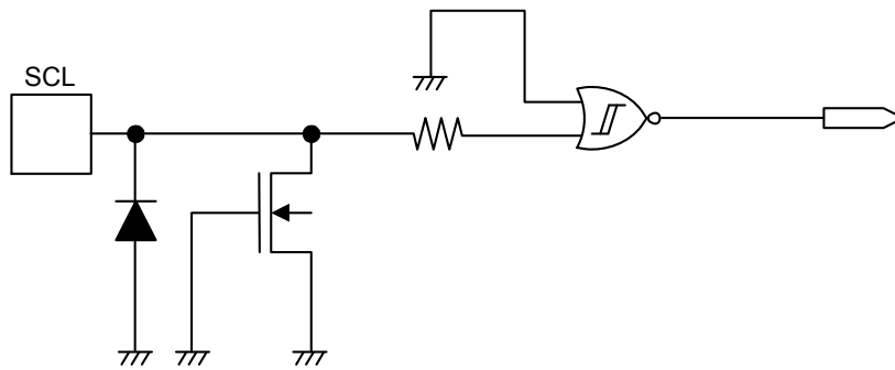
Figure 19 SCL Pin
