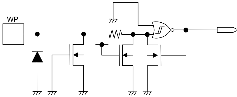
Figure 21 WP Pin
