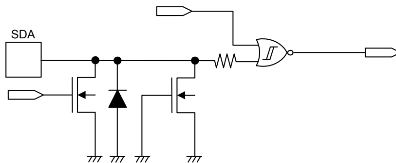
Figure 20 SDA Pin
