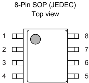
Figure 1 S-24CM01CI-J8T1U4
