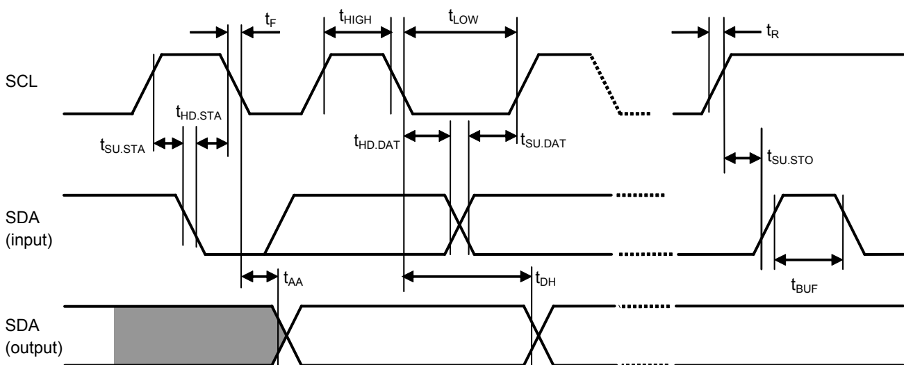
Figure 4 Bus Timing
