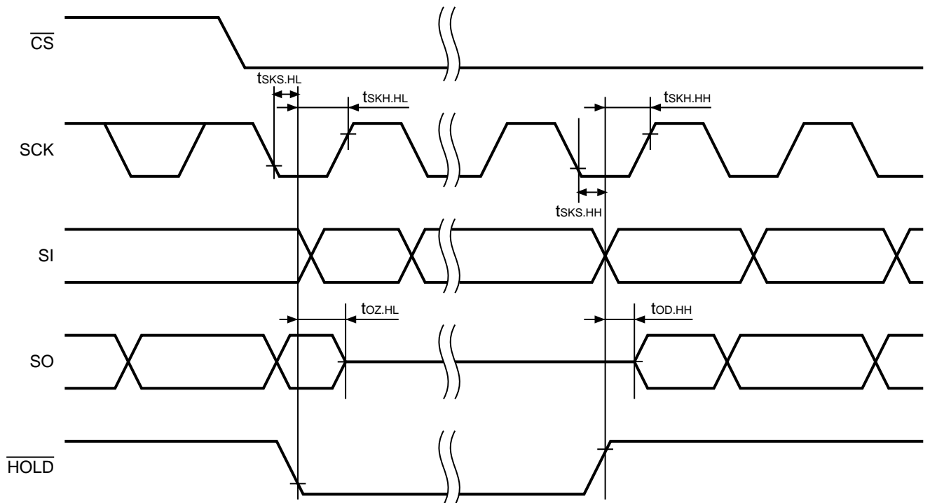
Figure 4 Hold Timing
