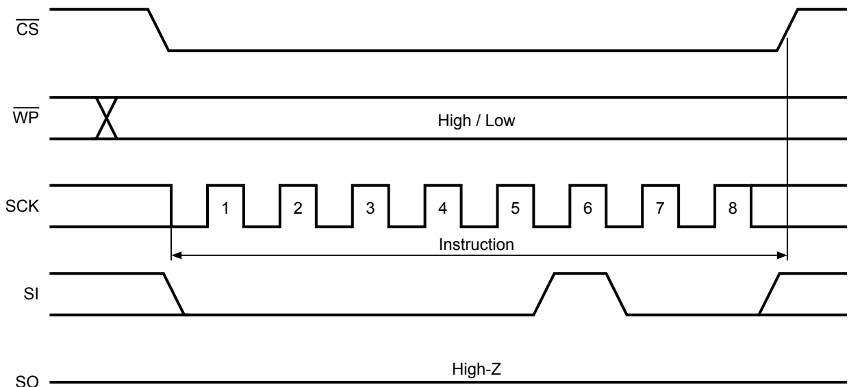
Figure 13 WRDI Operation
