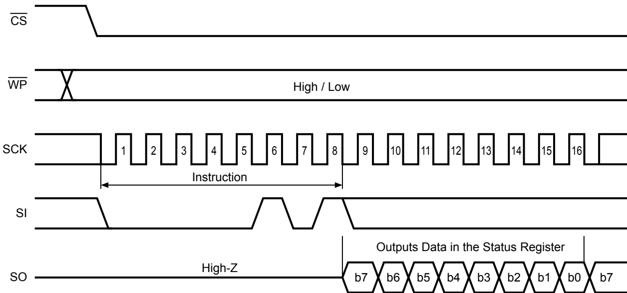
Figure 14 RDSR Operation
