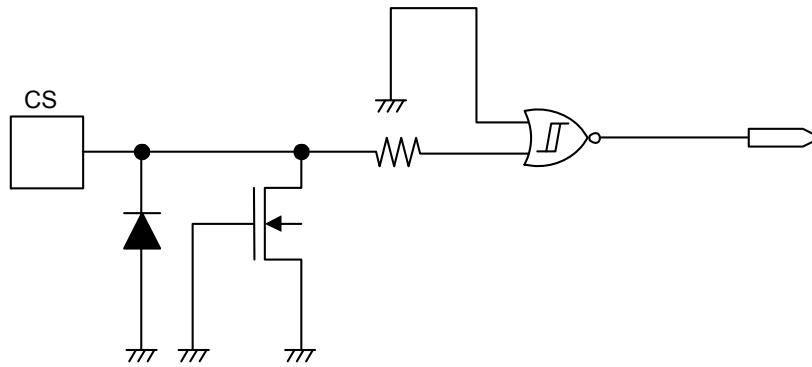
Figure 21 CS Pin
