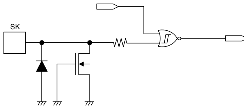
Figure 22 SK Pin
