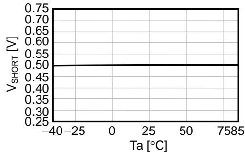
(10) V_{SHORT}-T_a
