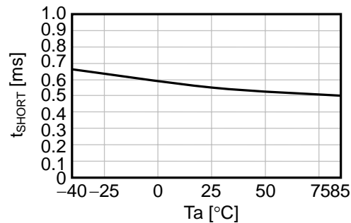
(12) t_{SHORT}-T_a
