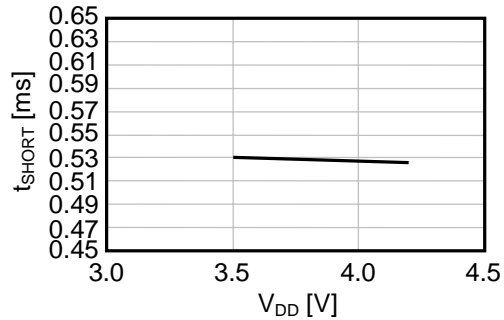
(11) t_{SHORT}-V_{DD}
