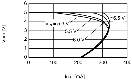
S-1323B50 (Ta=25°C)
