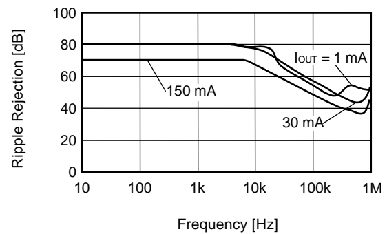
S-1323B30 (Ta=25°C)
